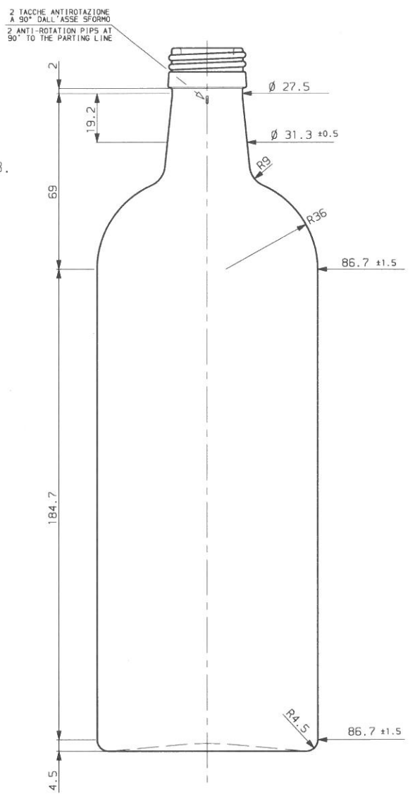
VISTA IN DIAGONALE MINOR AXIS VIEW
